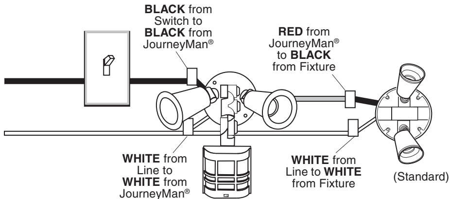
Wiring to a Motion Light & Standard Fixture
